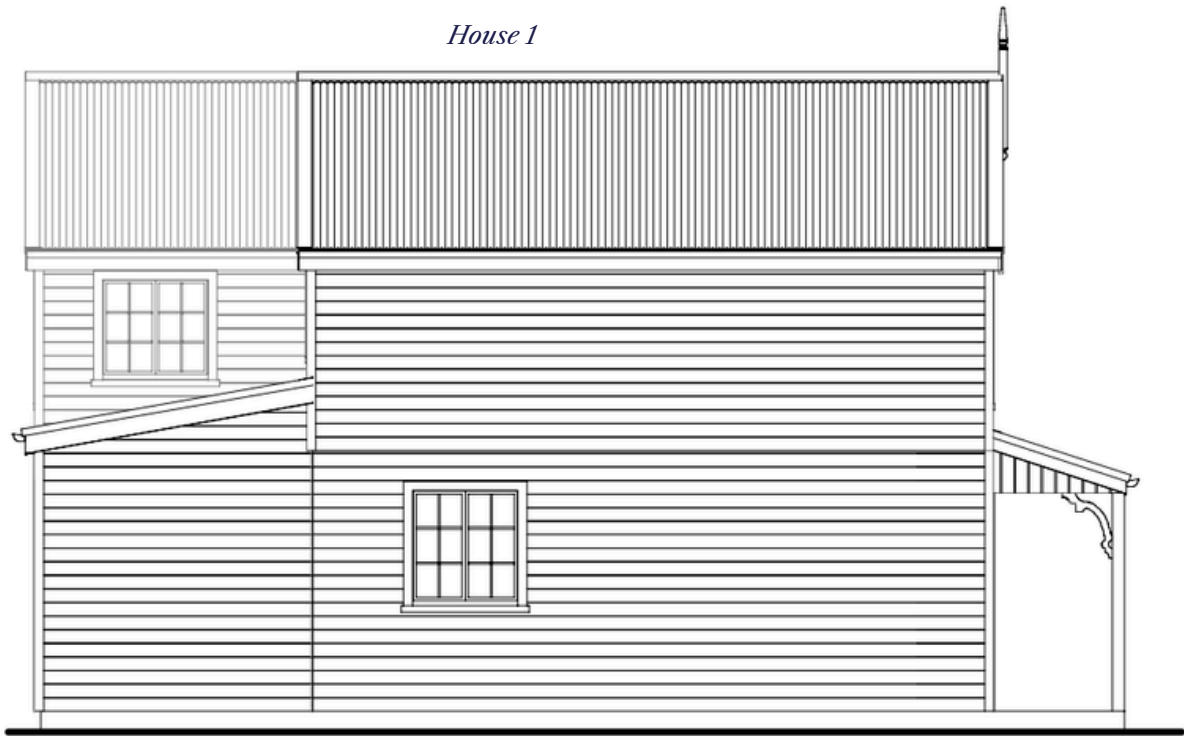
West Elevation
