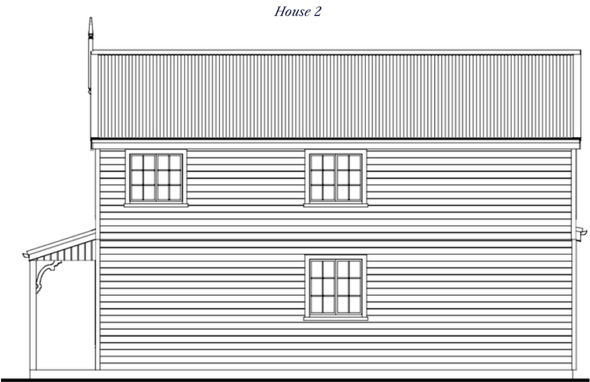
East Elevation
