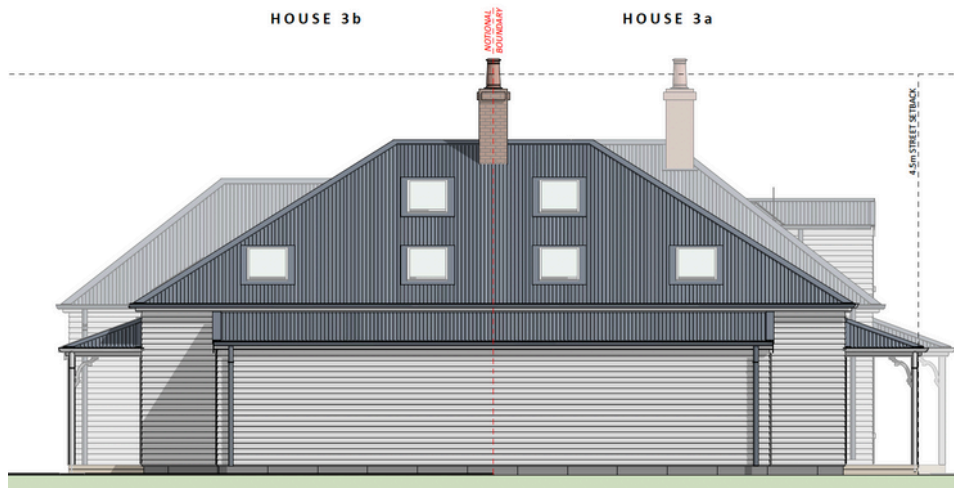
South Elevation
